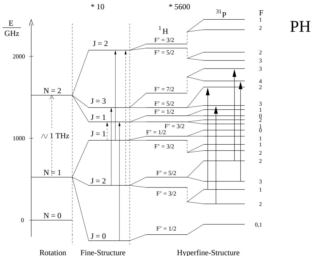
Fig. 2. Section of the energy level diagram of PH ( \Sigma^- ). The fine structure terms are enlarged 10 times. Bold arrows mark observed transitions with higher intensity ( \Delta J = 1 ), dotted arrows mark observed transitions with lower intensity ( \Delta J = 0 ). The hyperfine structure contributions of ^1\text{H} and ^{31}\text{P} are enlarged 5600 times. Both recorded transitions in Fig. 1 ( F_1 = 2.5 \leftarrow 1.5 and F_1 = 3.5 \leftarrow 2.5 ) are split further by the phosphorus nucleus into neighboring doublets, which experimentally are not observed. Here we emphasize that this interpretation of the observed splitting depends on the order of the coupling scheme of the nuclear spins as noted in the text. The observed splitting thus could equally well be interpreted as caused by the phosphorus nucleus.
